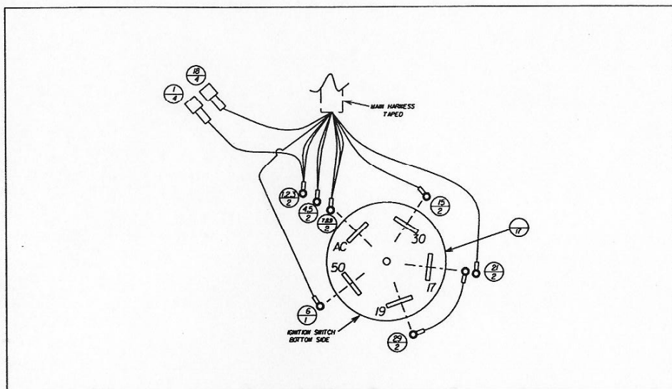
IGNITION SWITCH DIAGRAM
